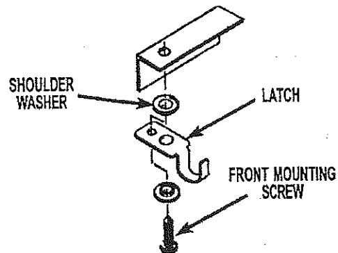
MISCELLANEOUS PARTS BAG (Part No. 685427)
