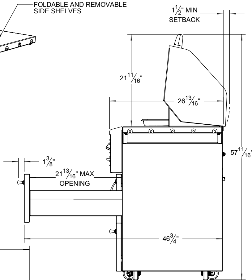
ALX2-30SZ SHOWN ON AL-30CD DELUXE CART
