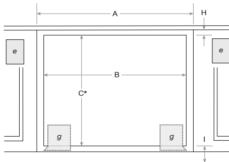
UNDER COUNTER INSTALLATION (without cooktop installed above)
