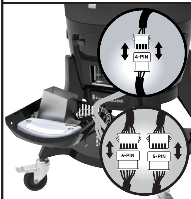
Disconnect the wire harness from the front module. Use caution do not apply tension on the wire harness.
