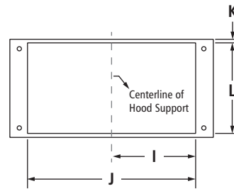
CUTOUT VIEW
